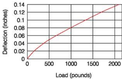
AT-300 Distributed Load Chart
