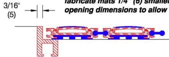
Recessed frame ATF-1002 (see ED.1.0) or ATF-1005 (see ED.2.0)
