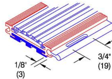
Perforated hinge
