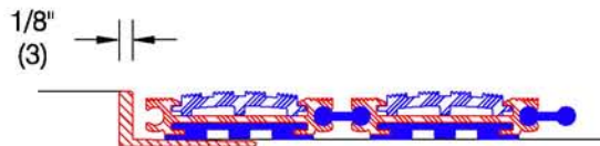
Recessed frame ATF-125 (see ED.3.0)
