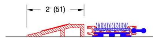
Surface frame ATF-225 (see ED.4.0)
