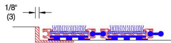
Recessed frame ATF-125 (see ED.3.0)
