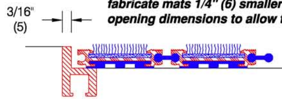
Recessed frame ATF-1002 (see ED.1.0) or ATF-1005 (see ED.2.0)
