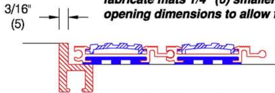
Recessed frame ATF-1002 (see ED.1.0) or MRF-1005 (see ED.2.0)
