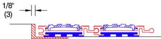
Recessed frame ATF-125 (see ED.3.0)
