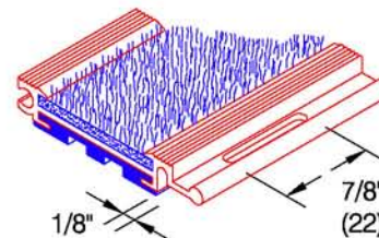
Optional perforated hinge (solid hinge standard)
