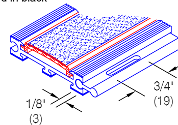
Perforated hinge
