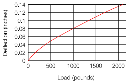
G-300 Distributed Rolling Load
