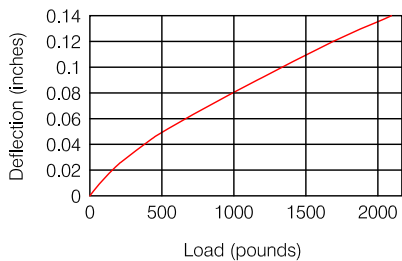
G-300 Distributed Load Chart
