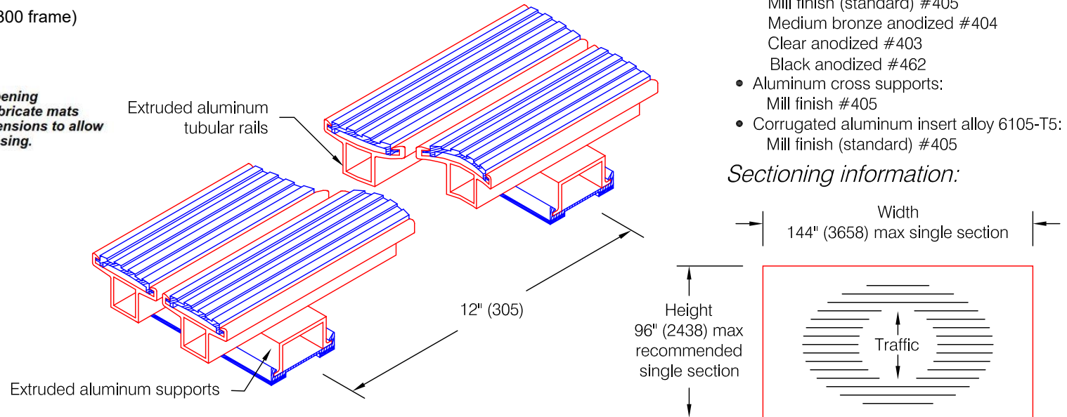
G-300 Distributed Rolling Load
