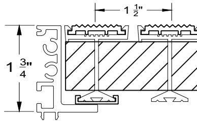
GF-740C Cast-in level-bed
