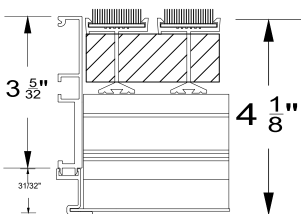
GF-740XD Cast-in extra deep-pit
