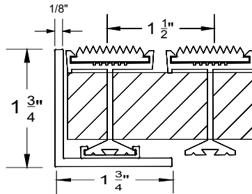
GF-740L Mechanically fastened level-bed
