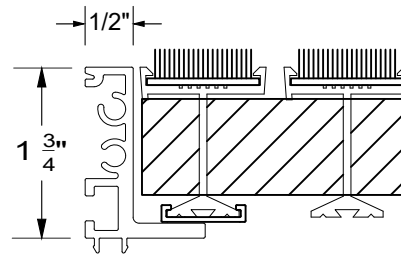
GF-740C Cast in level-bed
