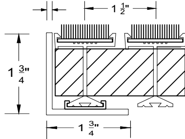
1/8" GF-740L Mechanically fastened level-bed
