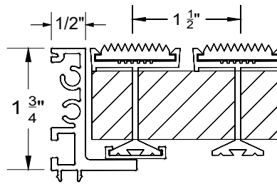
GF-740C Cast in level-bed
