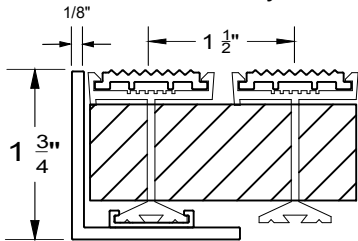
GF-740L Mechanically fastened level-bed
