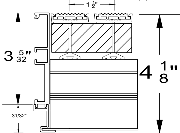
GF-740XD Cast-in extra deep-pit
