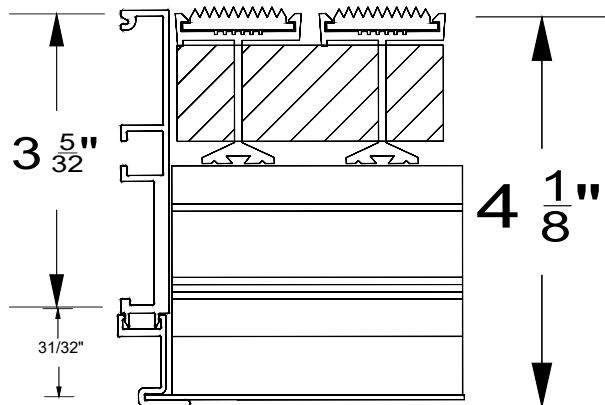
GF-740XD Cast-in extra deep pit
