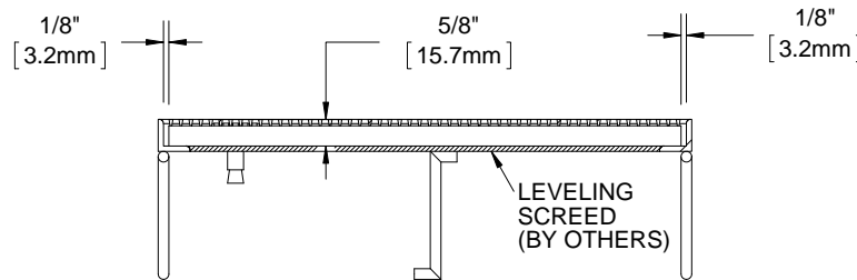
SECTION Y-Y
